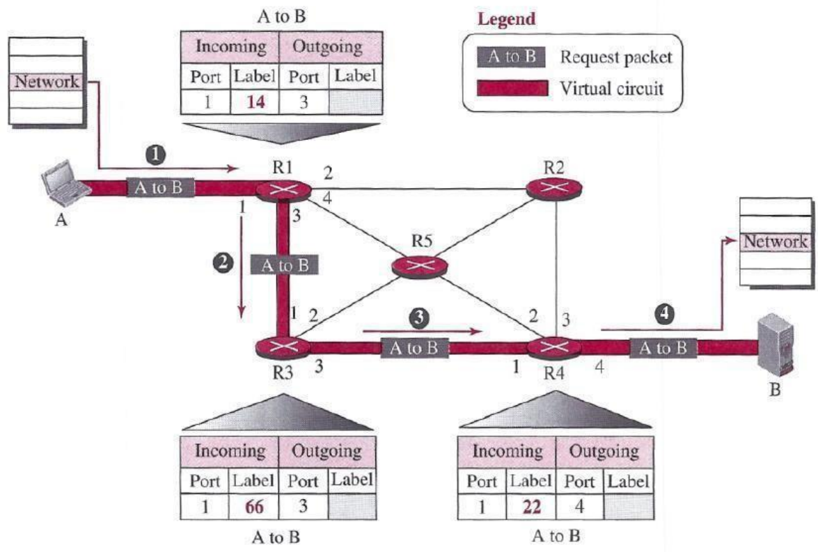
Sending request packet in a virtual-circuit network
