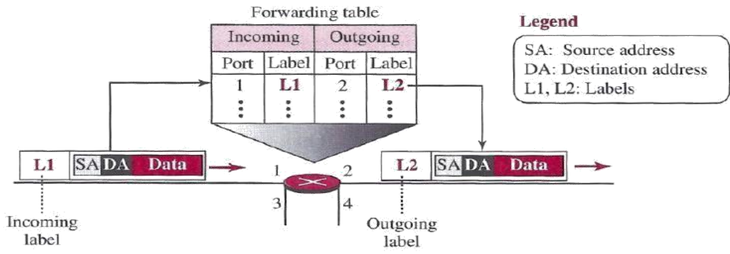
Forwarding process in a router when used in a virtual-circuit network
