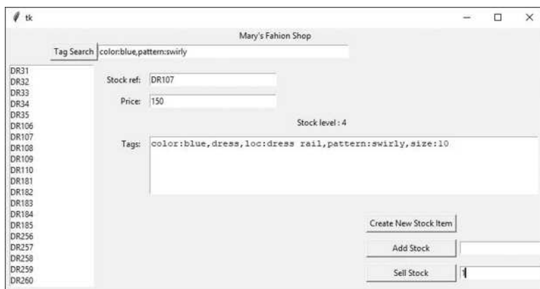
Figure 13-23 A Fashion Shop application with a graphical user interface
