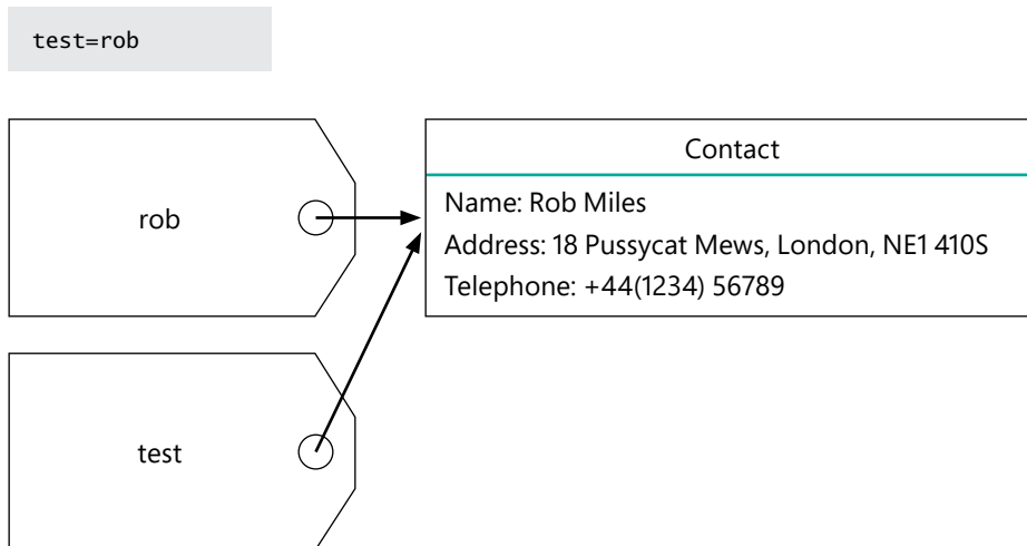
Figure 9-2 Two references to the same contact
