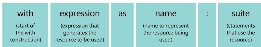
Figure 8-3 Anatomy of a with construction
