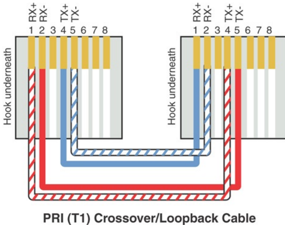
FIGURE 5.14 Pinouts for a T1 crossover cable
