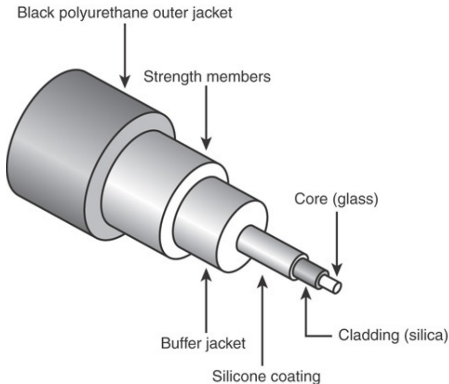
FIGURE 5.4 Fiber-optic cabling
