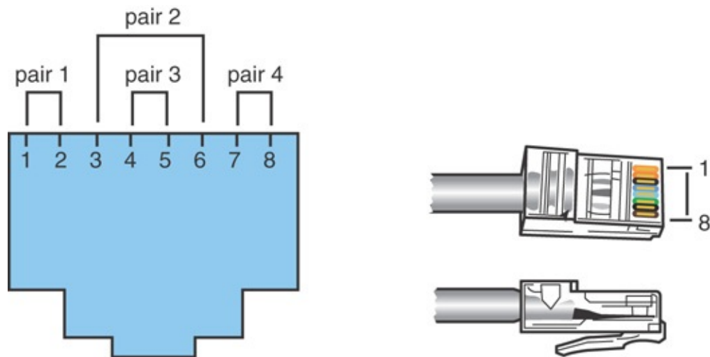
FIGURE 5.7 RJ-45 connectors
