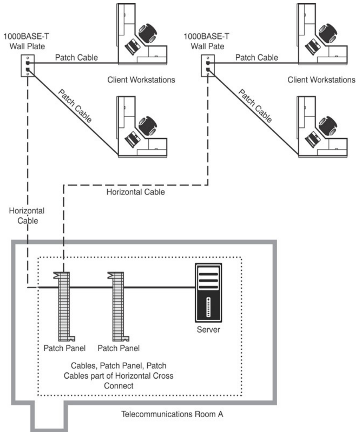
FIGURE 5.15 Horizontal cabling
