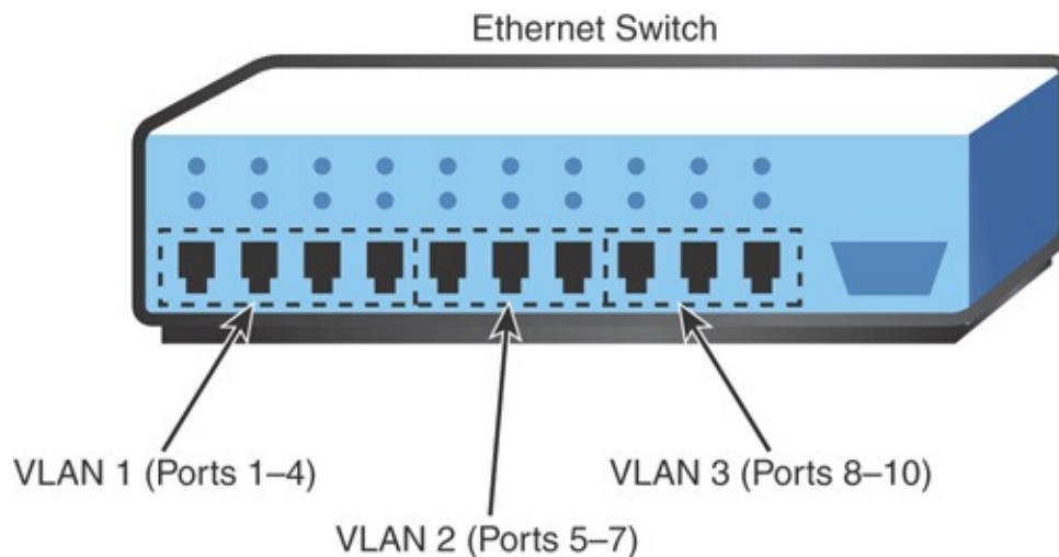
FIGURE 3.7 Port-based VLAN membership
