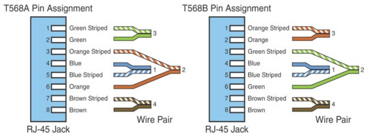
FIGURE 5.11 Pin assignments for the T568A and T568B standards
