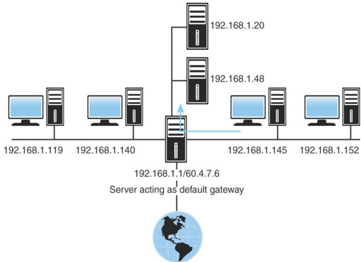
FIGURE 3.1 The role of a default gateway
