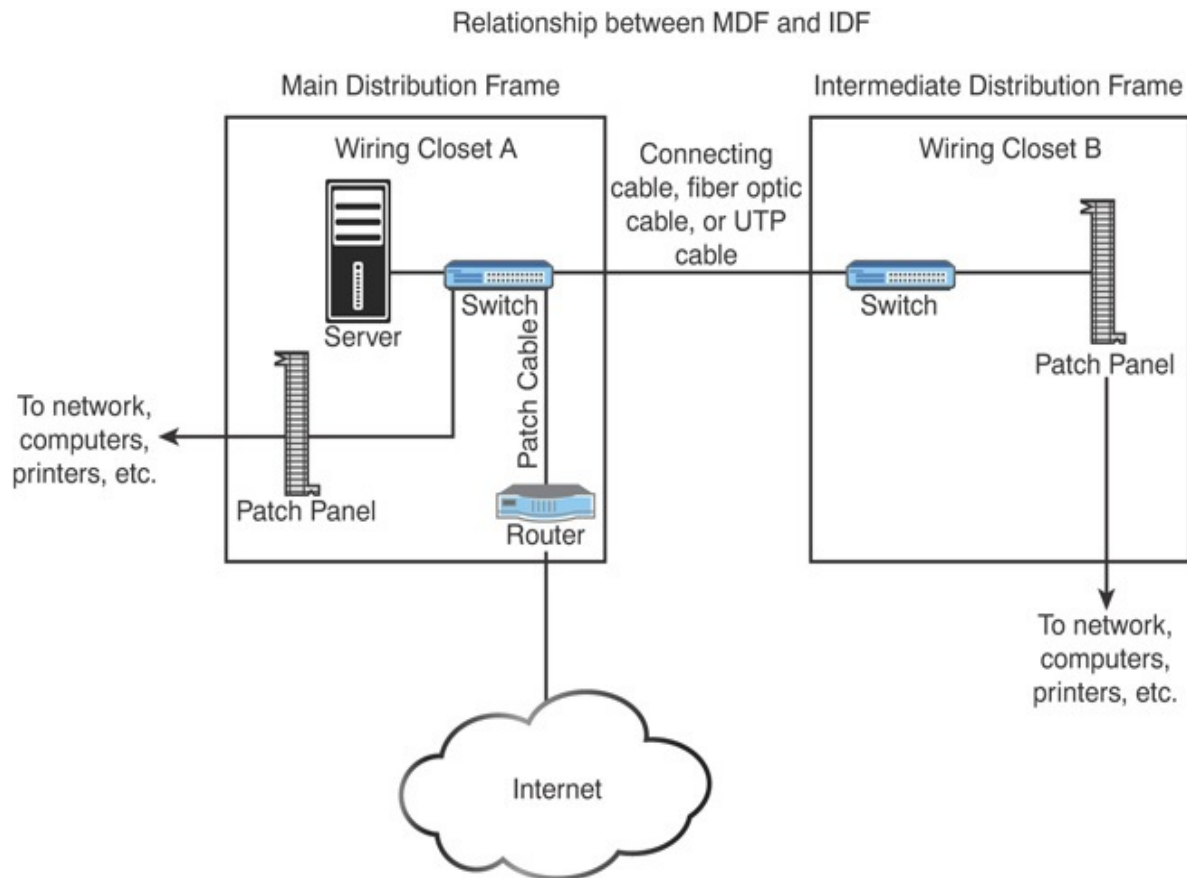
FIGURE 5.18 The relationship between MDFs and IDFs
