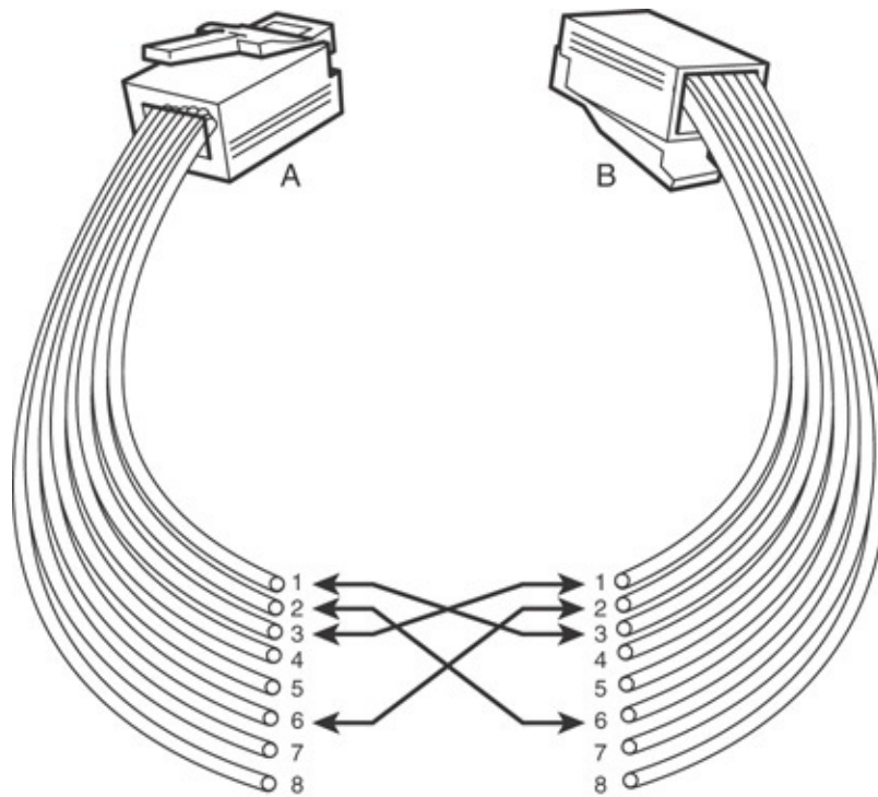
FIGURE 5.13 Pinouts for a crossover twisted-pair cable
