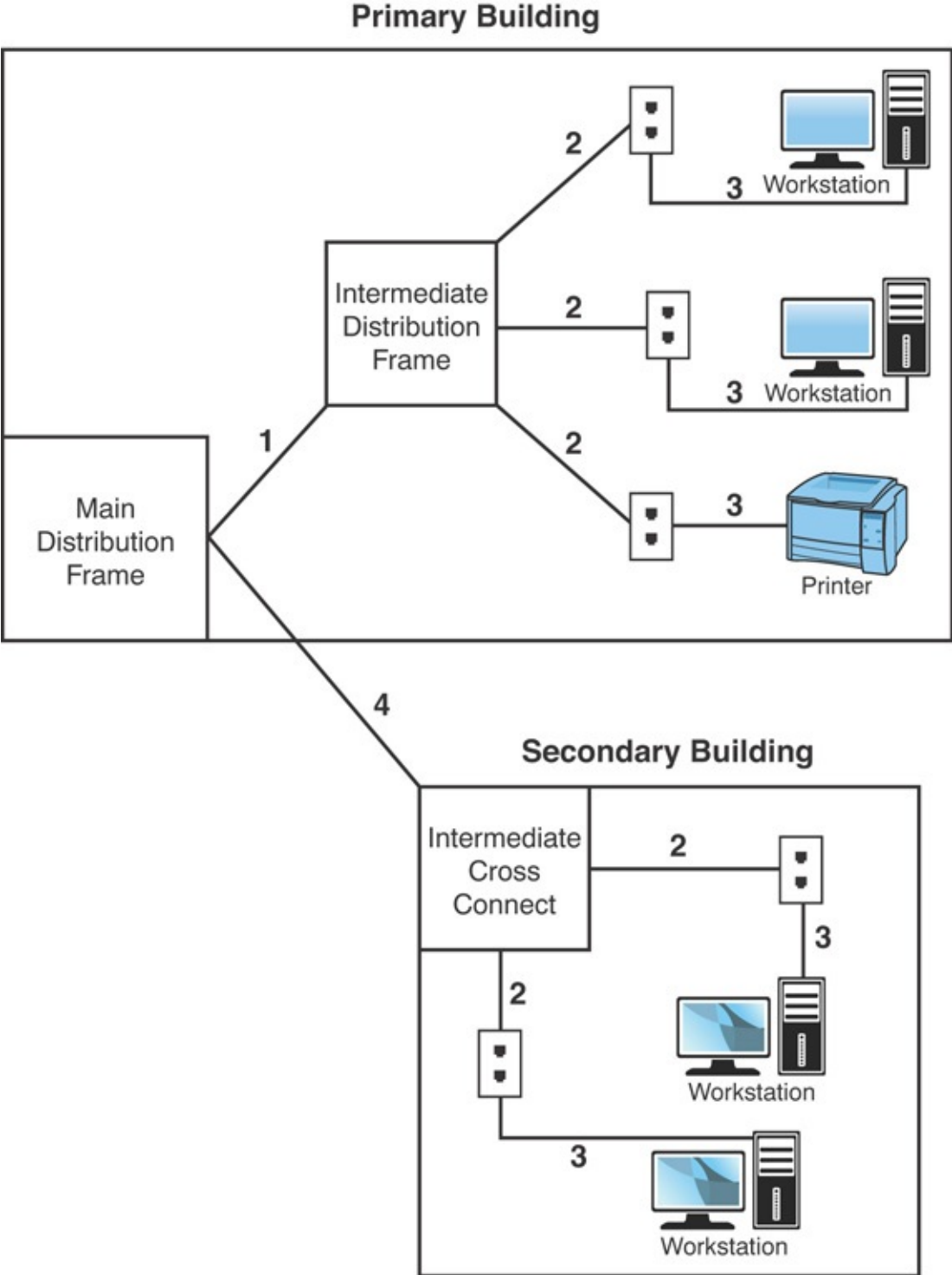
FIGURE 8.2 A general wiring schematic
