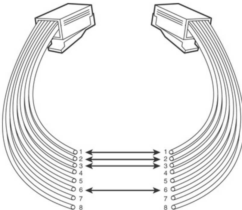
FIGURE 5.12 Pinouts for a straight-through twisted-pair cable
