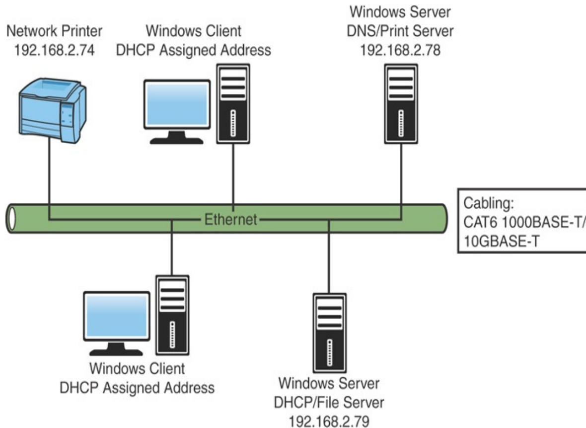
FIGURE 8.3 A physical network diagram
