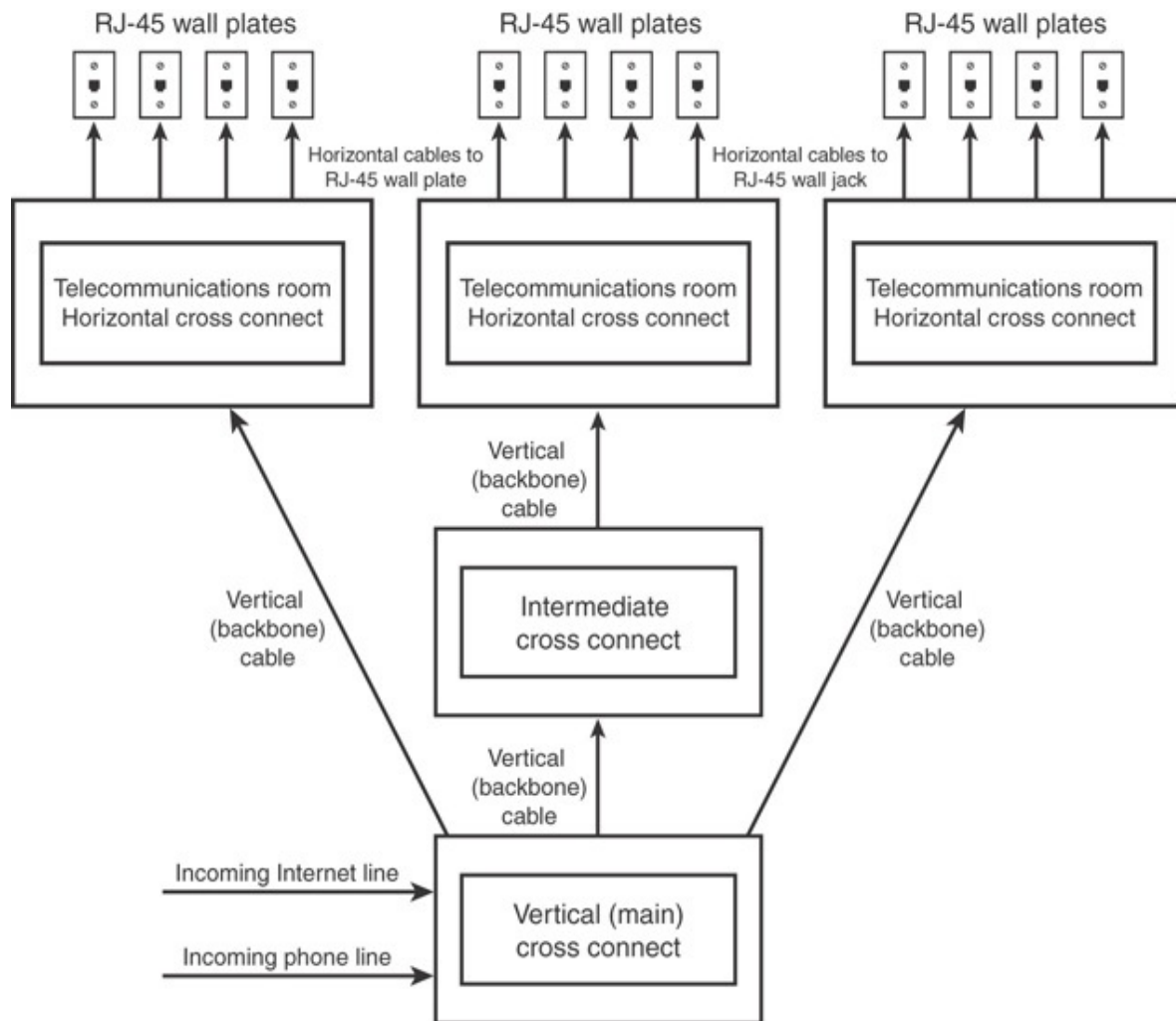
FIGURE 5.16 Vertical and horizontal cabling
