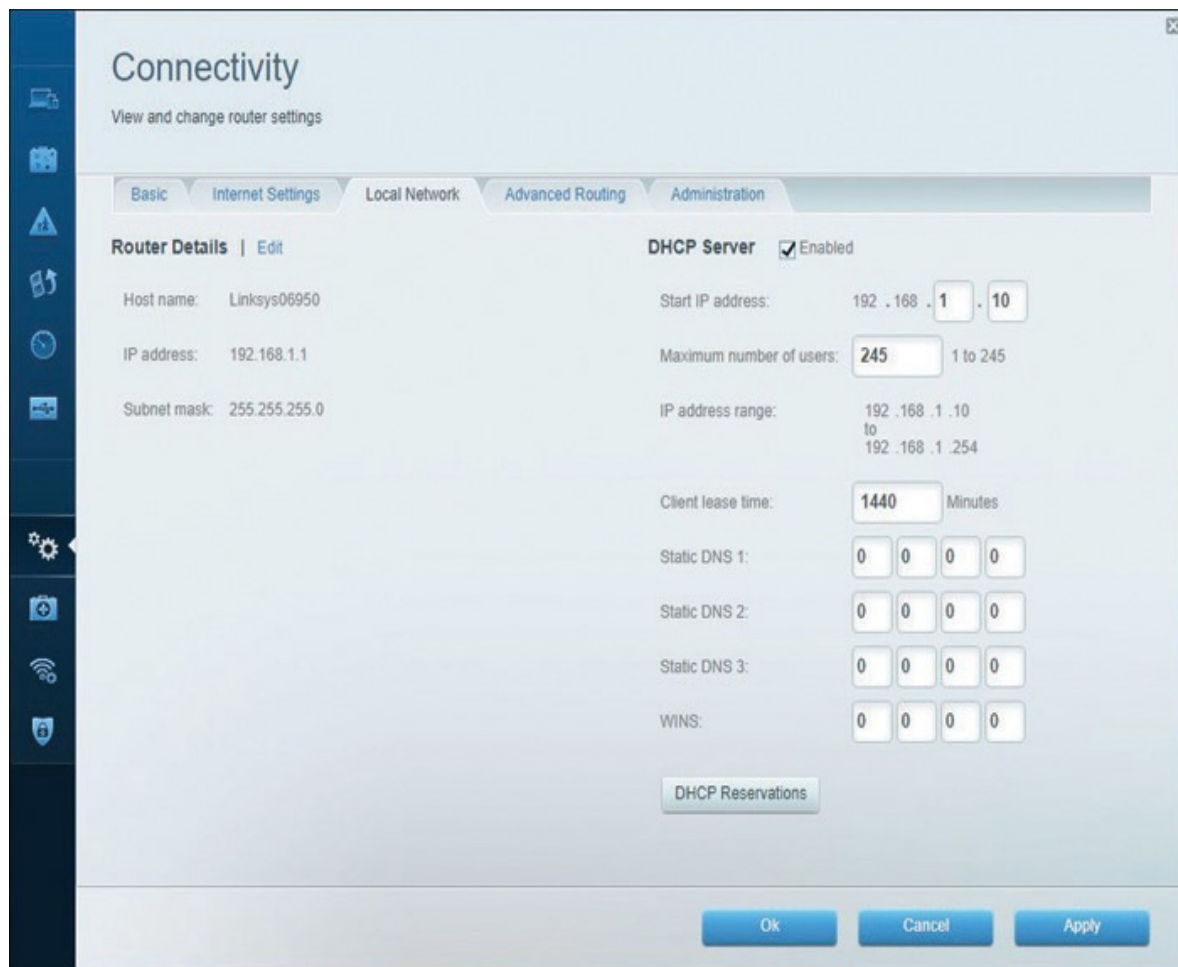
FIGURE 2.3 Configuring DHCP on a SOHO router
